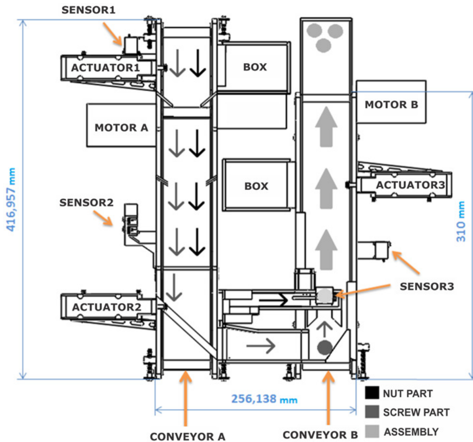
Figure 1. Assembly plant
