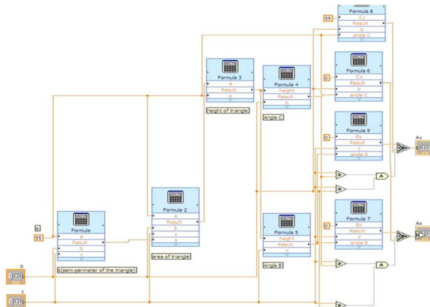
Figure 6: Head Distance Sub VI
