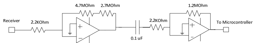
Figure 5: Custom Built Amplifier [1]
