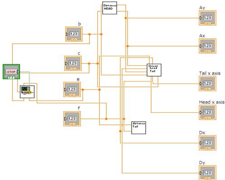
Figure 9: LabVIEW ultrasound Sub VI, with all distance and orientation calculations
