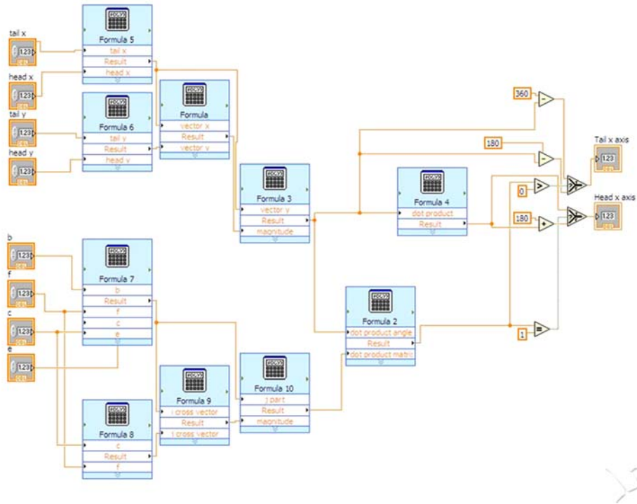
Figure 8: Orientation Sub VI
